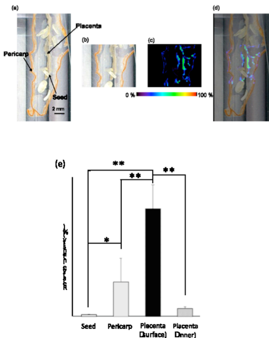
Figure 4: MALDI-TOF-MSI of capsaicin. Optical images of Capsicum sections (a). The MSI region of Capsicum (b). MS spectra reconstructed as ion images for m/z 306.2 (c). Merged image of optical Capsicum and MSI for m/z 306.2 (d). Total MS intensity at pericarp, seed and placenta of Capsicum fruits (e). These areas were measured to quantify the MS intensity, respectively. Obtained values were commuted to per unit area. The values are expressed in terms of mean \pm SEM. * P < 0.05 and ** P < 0.01 with Student's t -test. n=3 .
