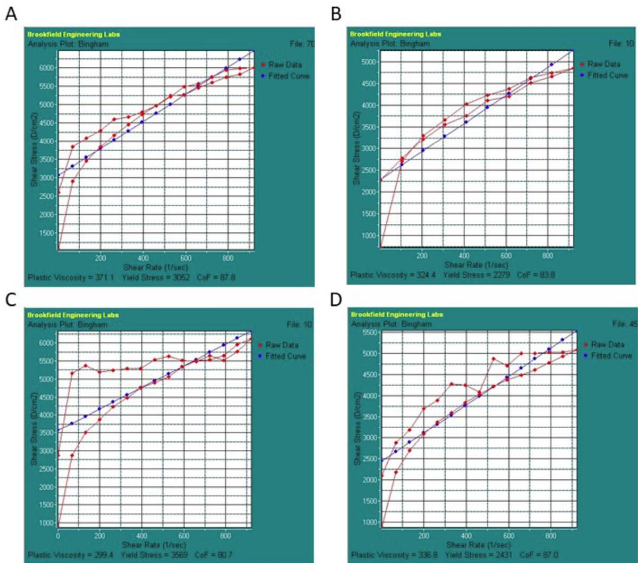
Figure S3: Rheogram profile of biopolymeric gels after 3 months stability. A) CS/AV/VC 1:1 in refrigerator, B) CS/AV/VC 1:1 in room temperature, C) CS/AV/VC 1:2 in refrigerator and D) CS/AV/VC 1:2 in room temperature.
